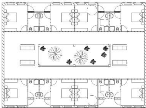
Plan R+1 type 1/100
