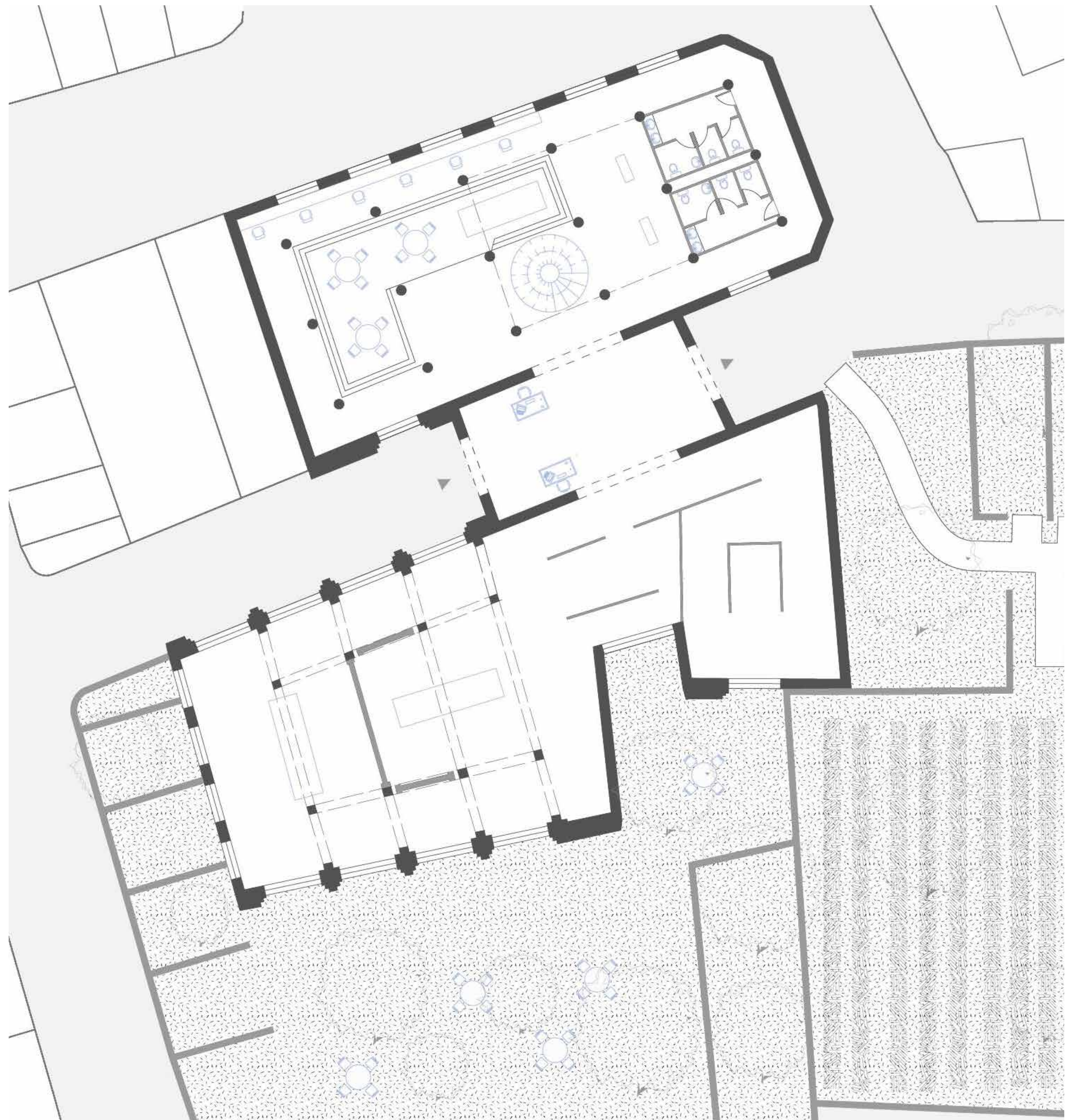
Library & Exhibition Hall Ground Floor 1:100
