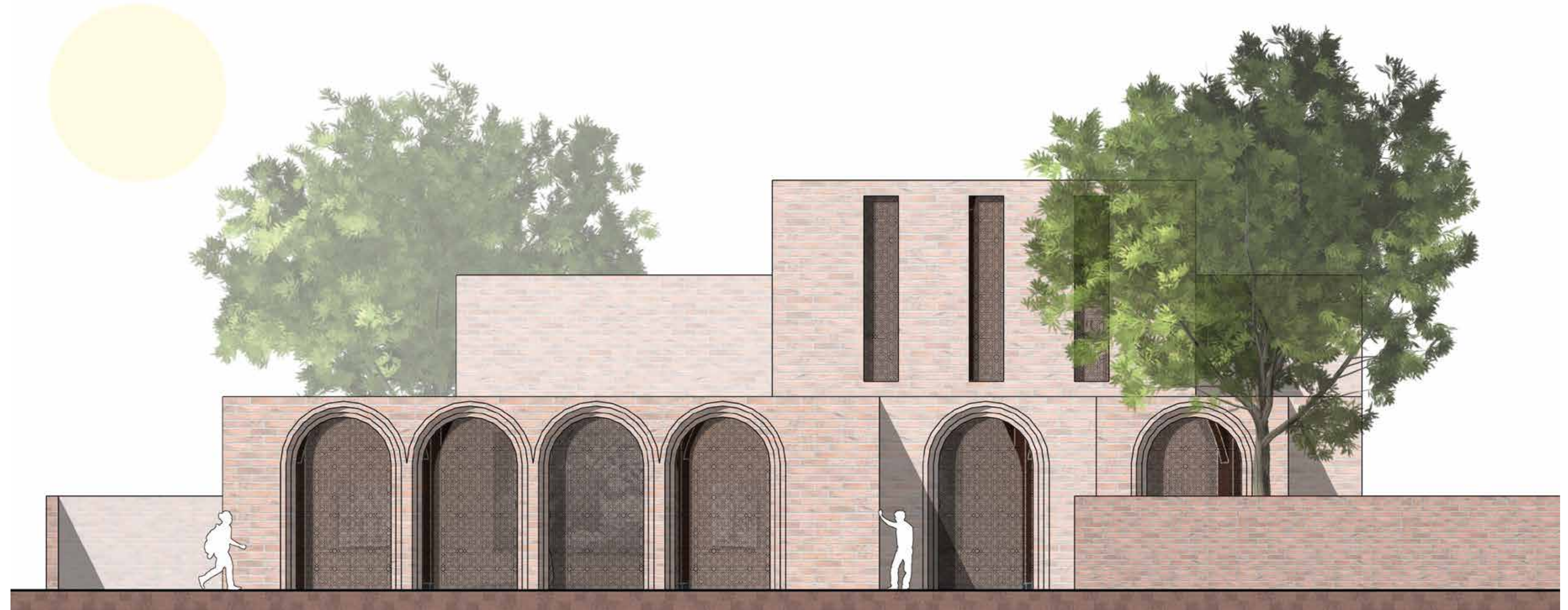
South Facade 1:100
